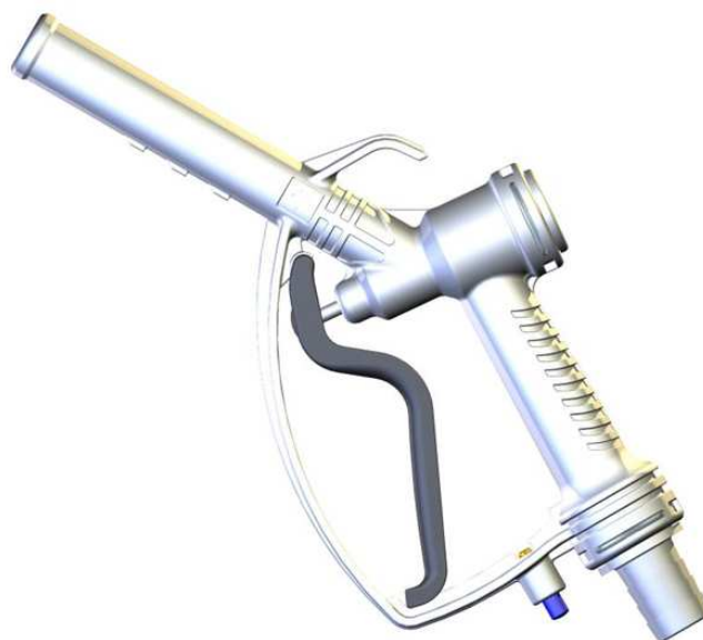
PMP120 B White Plastic Gun Transfer of Diesel Oil/Chemicals VITON Seals PP+FG+SS Inner Parts
